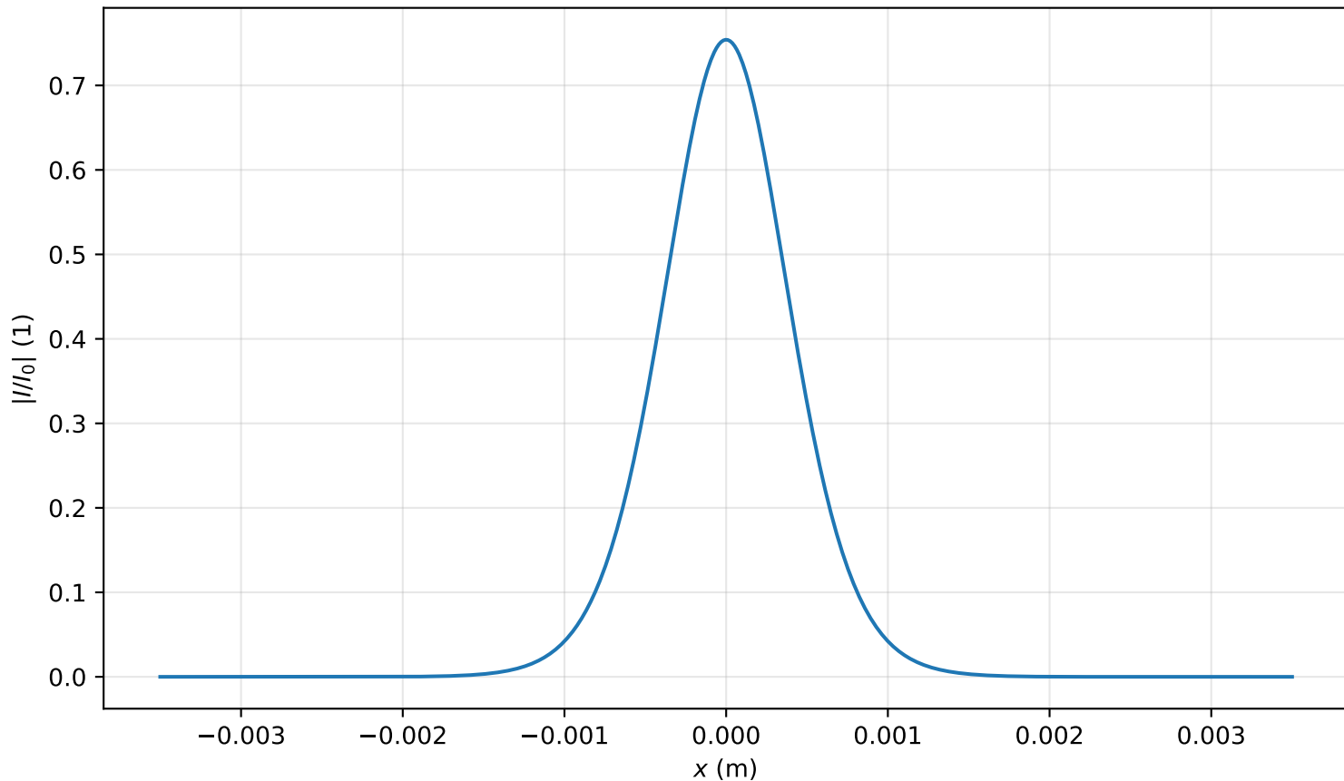
Intensity profile I(x, y = 0, z = 1.911m)/I_0 , P_{in}=0.4P_{cr} , artificial time
